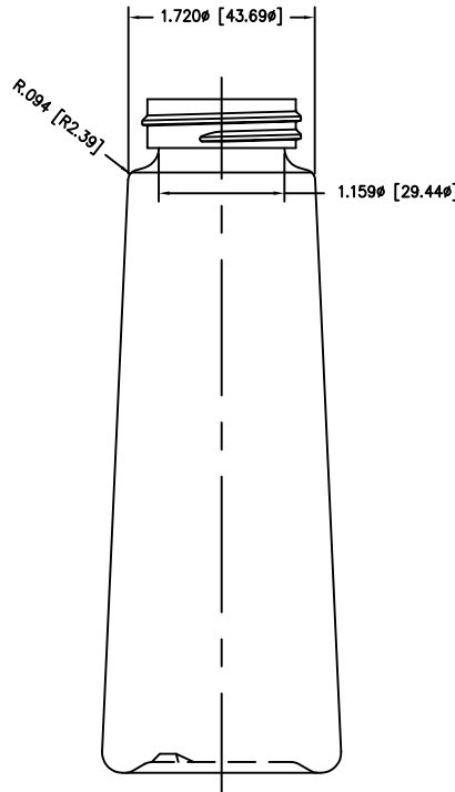
BACK VIEW
