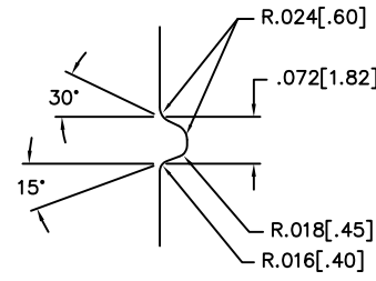
THREAD PROFILE SCALE: 5-1
