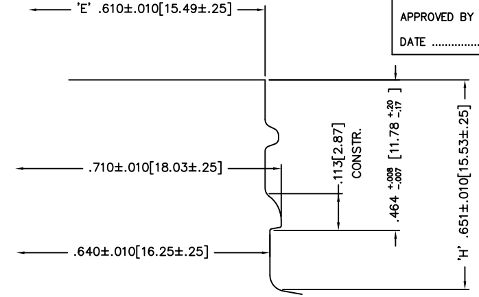
THREAD DETAIL SCALE: 4-1
